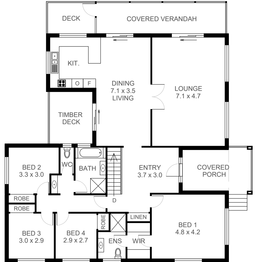
MAIN FLOOR PLAN ( 180 sq m Approx )
