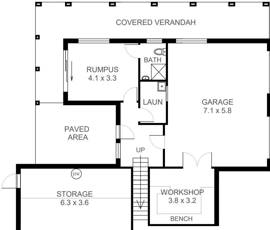
LOWER FLOOR PLAN ( 92 sq m Approx )
