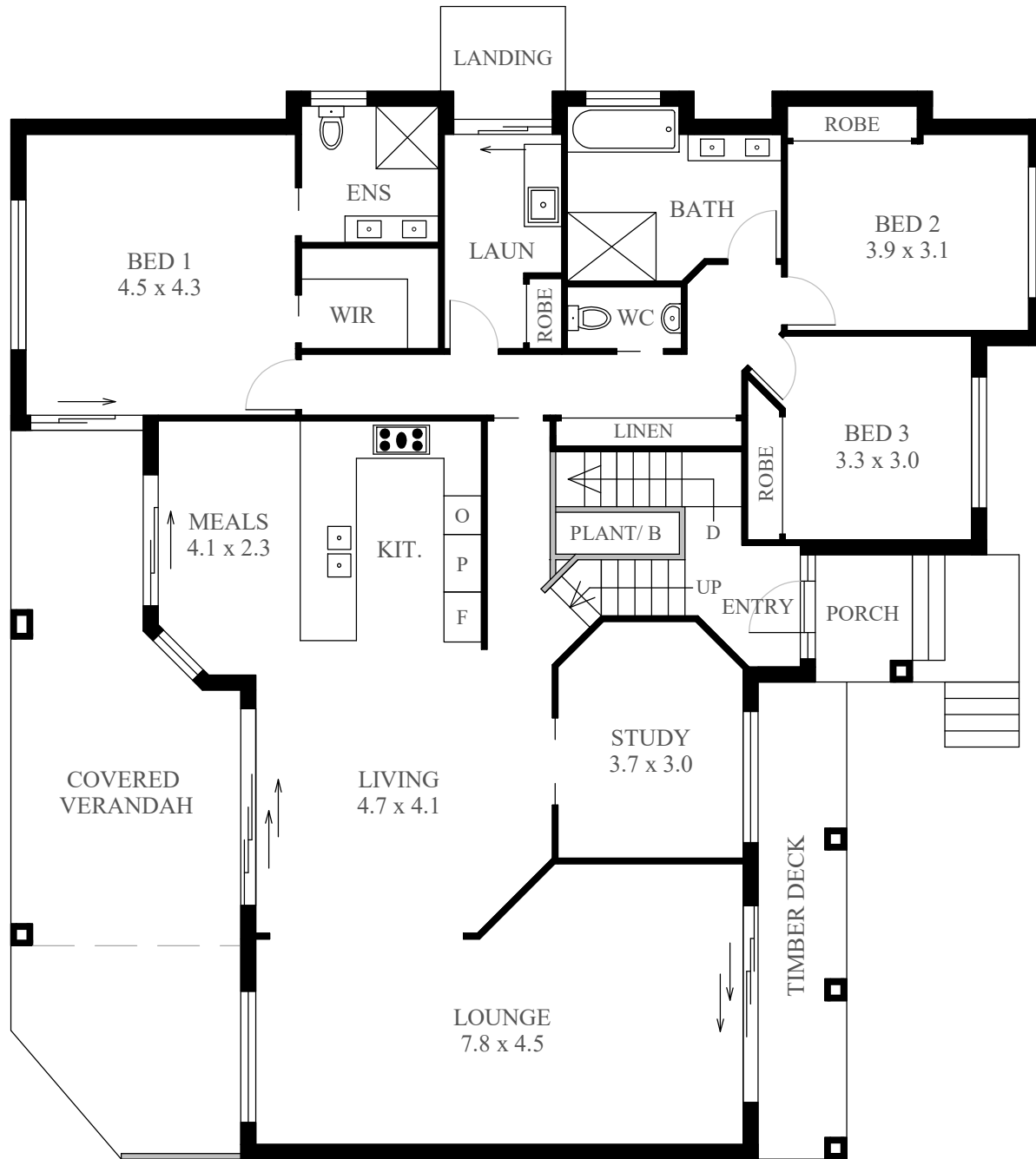
MAIN FLOOR PLAN ( 197 sq m Approx )
