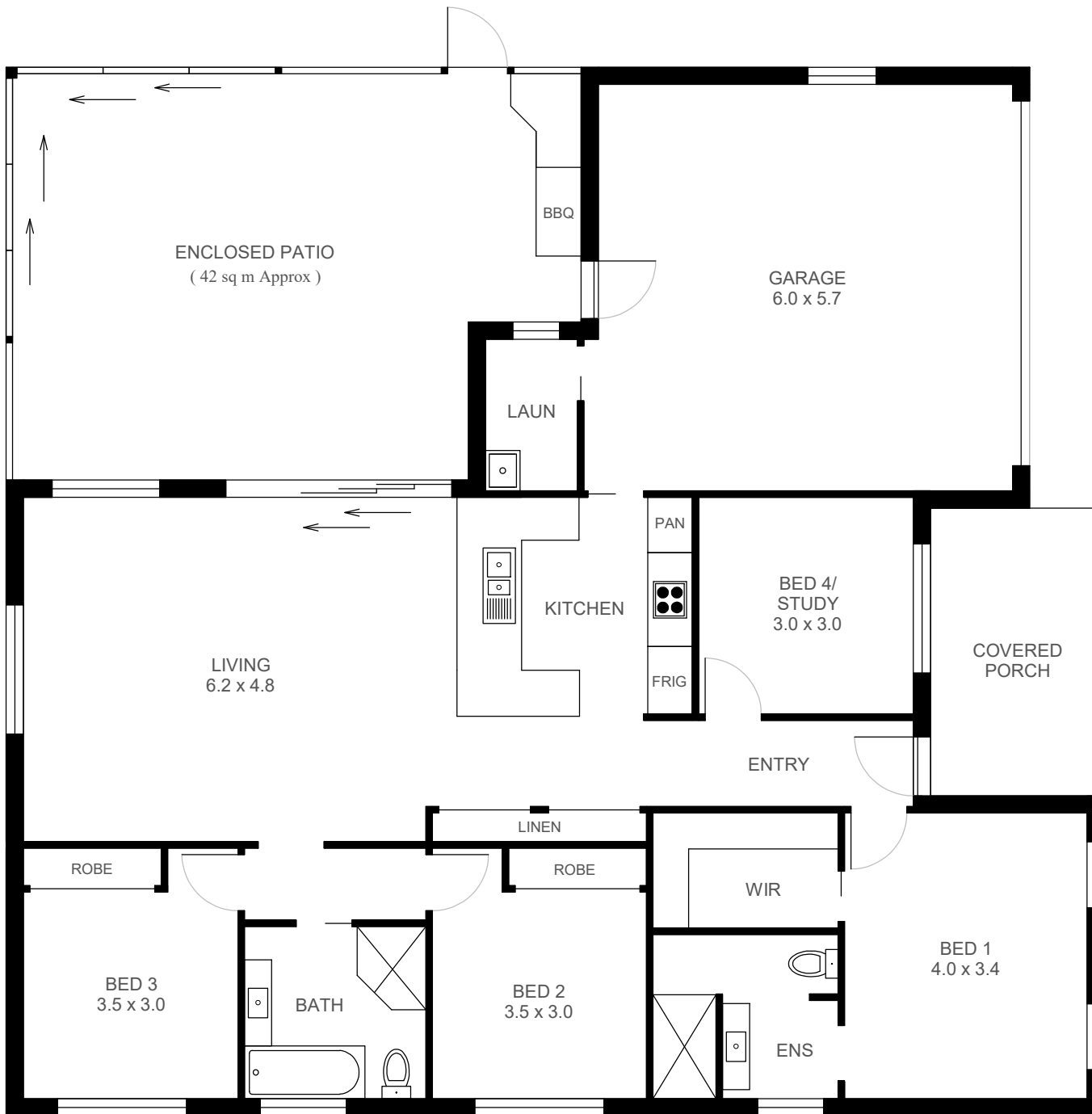
FLOOR PLAN ( 165 sq m Approx )
