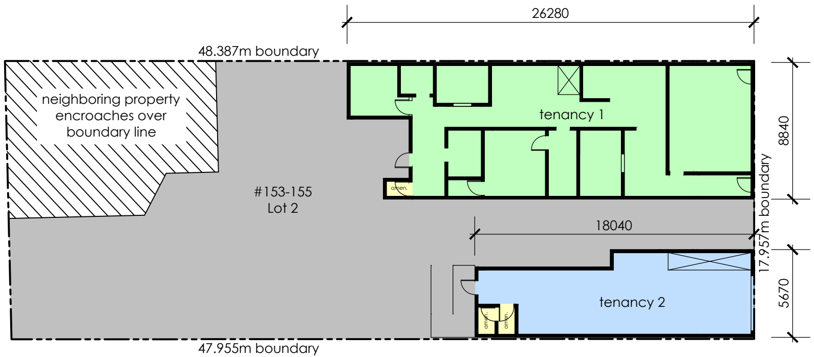
Site & Ground Floor plan
