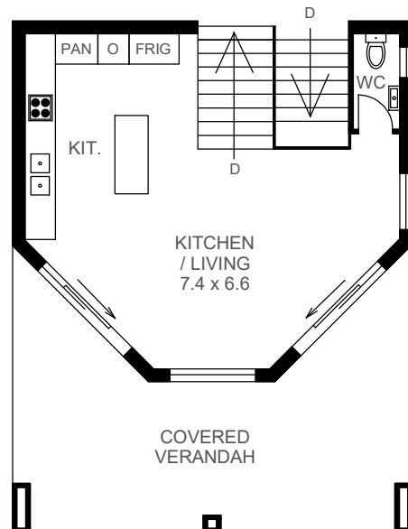
UPPER FLOOR PLAN ( 49 sq m Approx )
