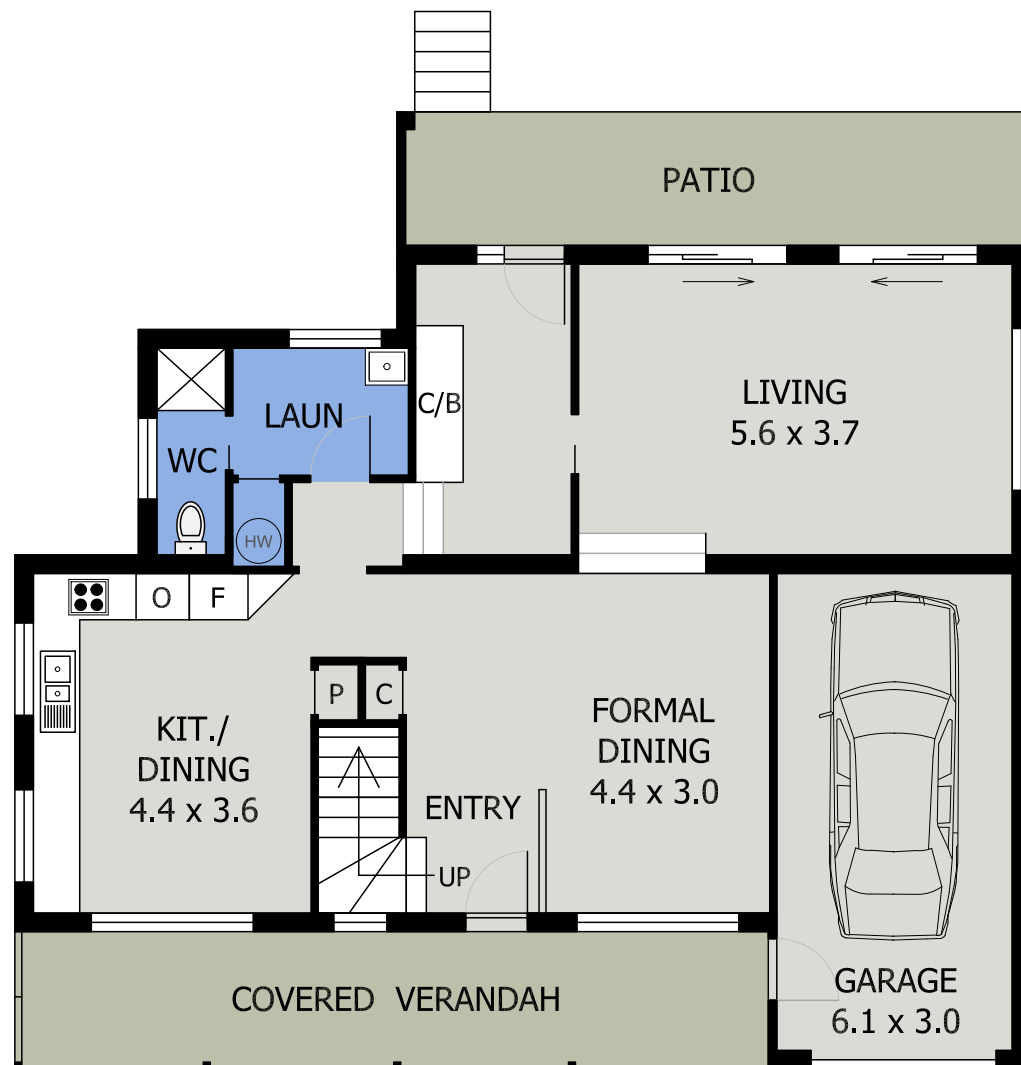
LOWER FLOOR PLAN
