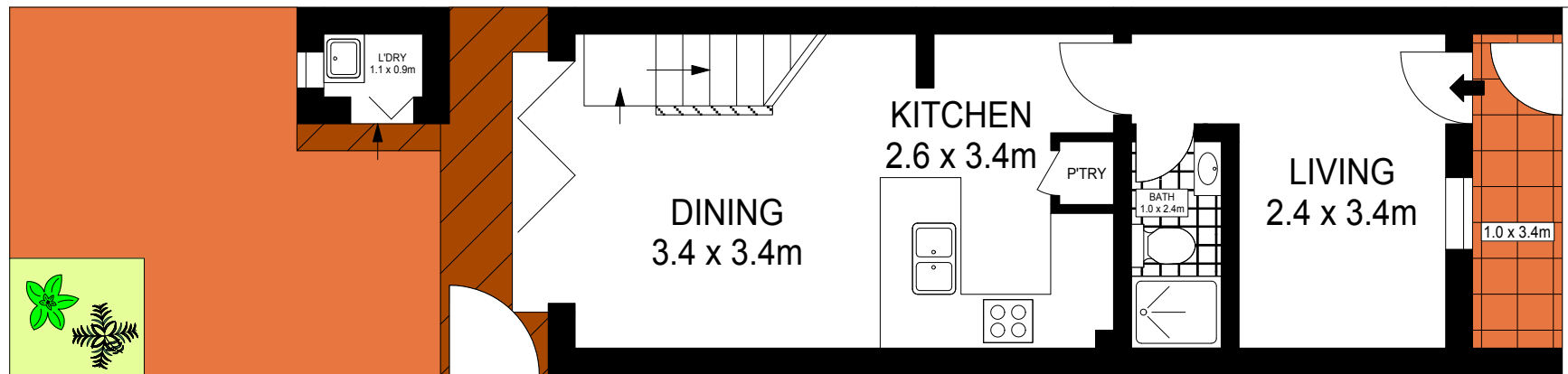
GROUND FLOOR
