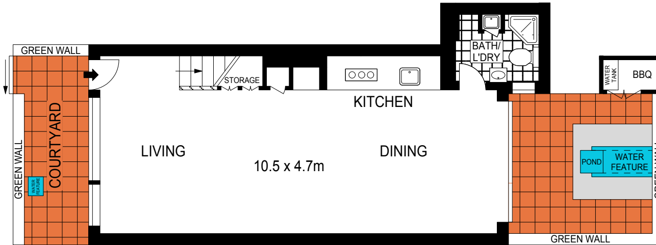
GROUND FLOOR
