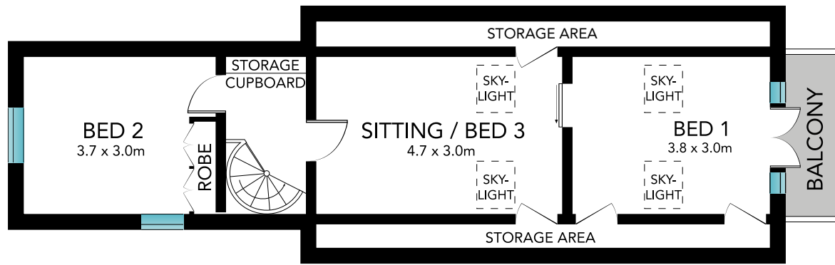
FIRST FLOOR
