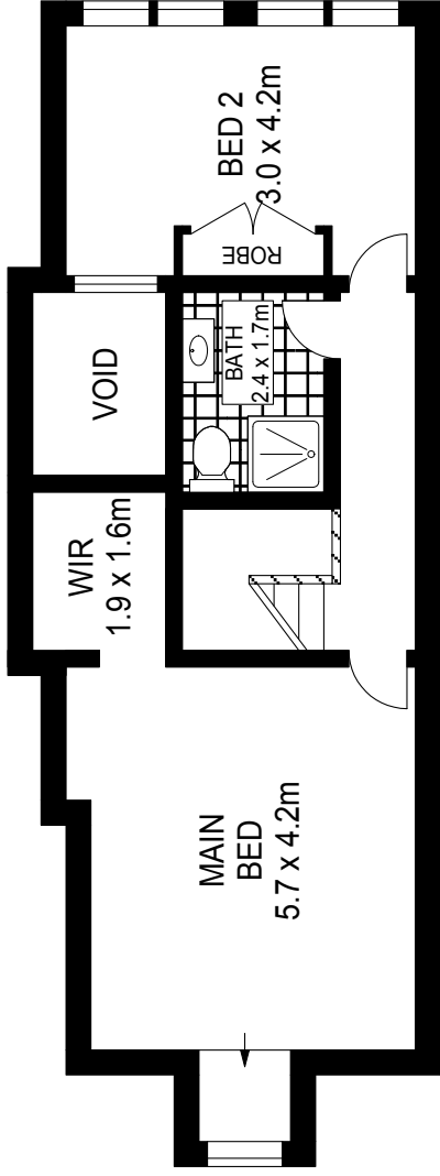
FIRST FLOOR
