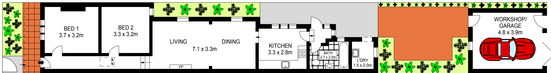
GROUND FLOOR
