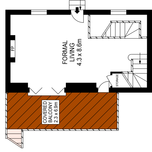
ENTRY LEVEL
