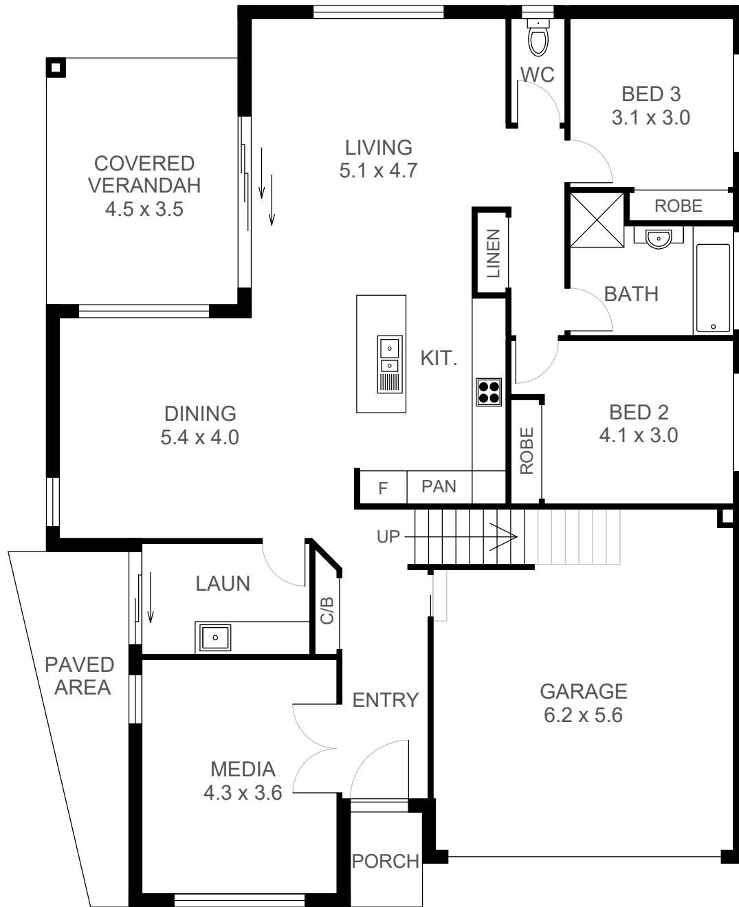
MAIN FLOOR PLAN ( 176 sq m Approx )
